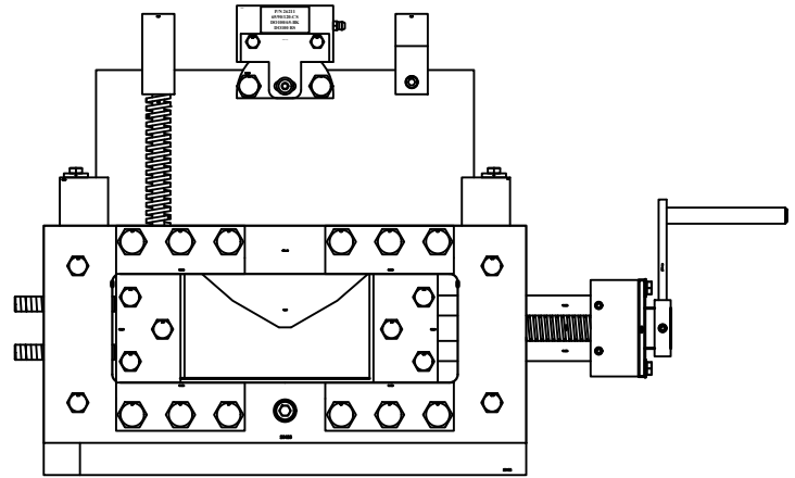
Channel Shear
