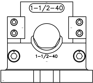
Pipe Notcher
