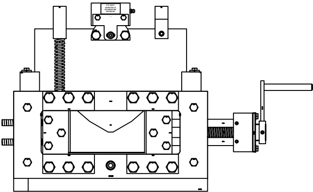
Channel Shear
