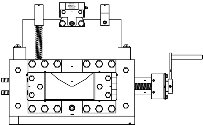
Channel Shear
