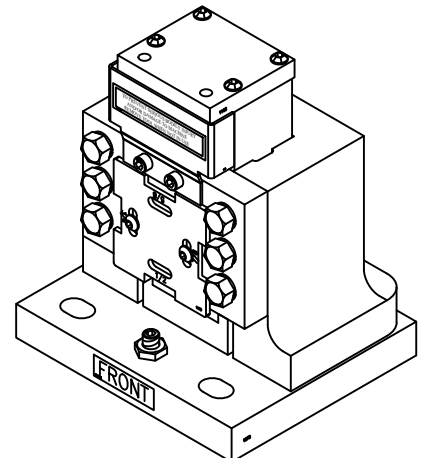
Picket Tool
